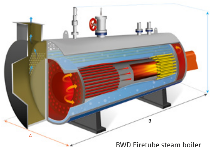
BWD Firetube steam boiler
